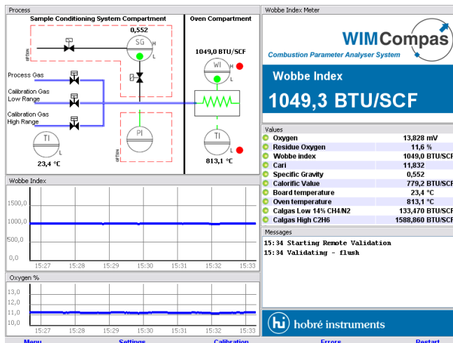
▲ Figure 4: WIM Compas F Display
